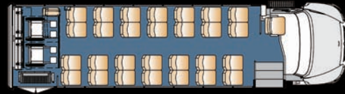
28 Passenger Plus 2 Wheelchair 2 Passenger Foldaway and 4 Passenger Flip Seats Plus Driver
